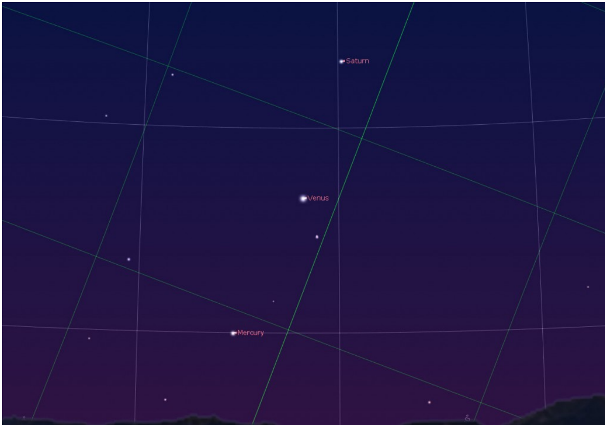
Night Sky in Giza, Egypt on December 3, 2012, local time ... one hour before sunrise. Image generated by Starry Night Pro.
